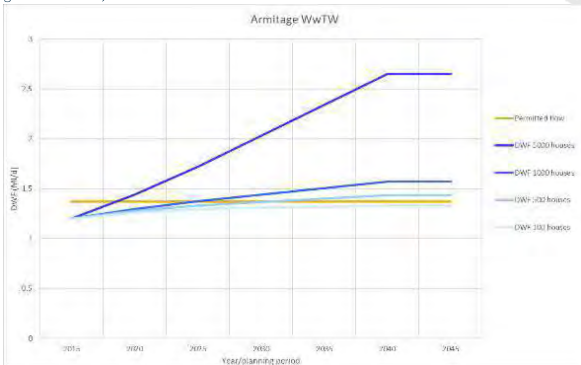
Figure 7-5 Flow permit assessment for Armitage WwTW (Lichfield preferred growth areas)
