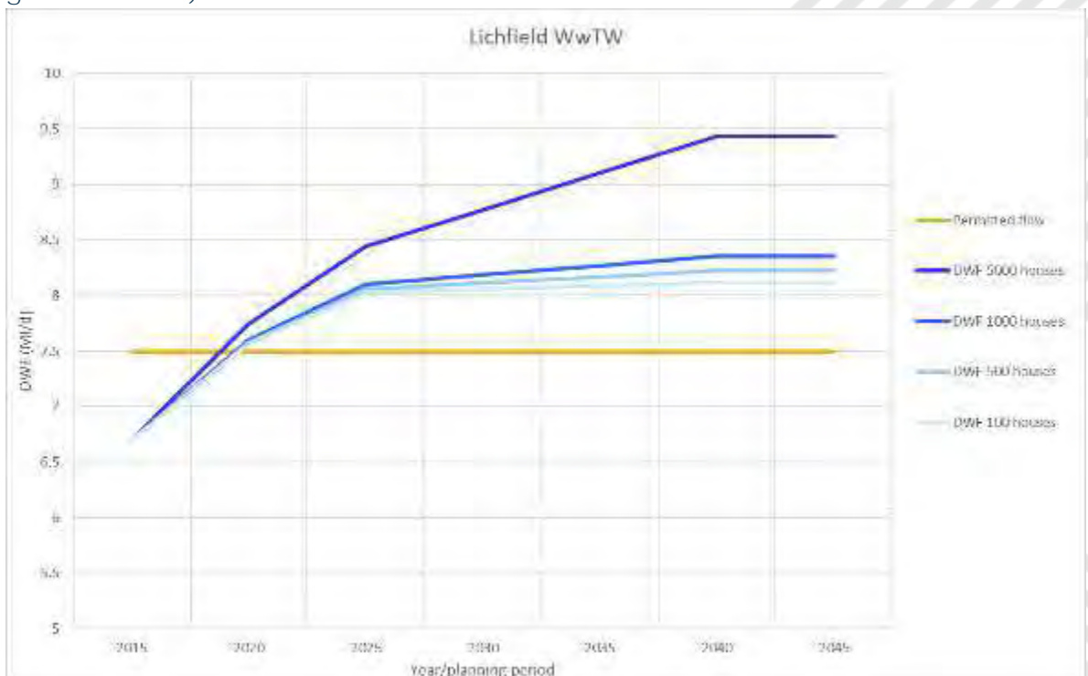
Figure 7-7 Flow permit assessment for Lichfield WwTW (Lichfield preferred growth areas)
